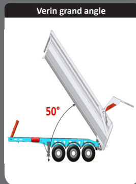
Verin grand angle
