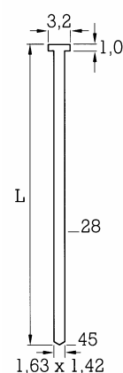
Pointe type SK 400
