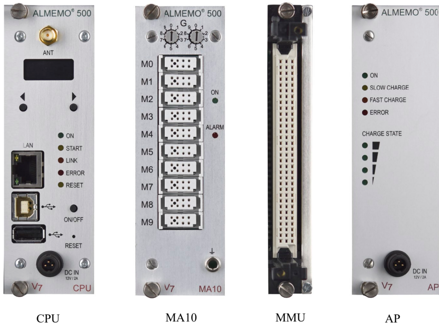
CPU
