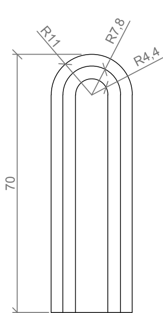
ALZADO / FRONT VIEW
