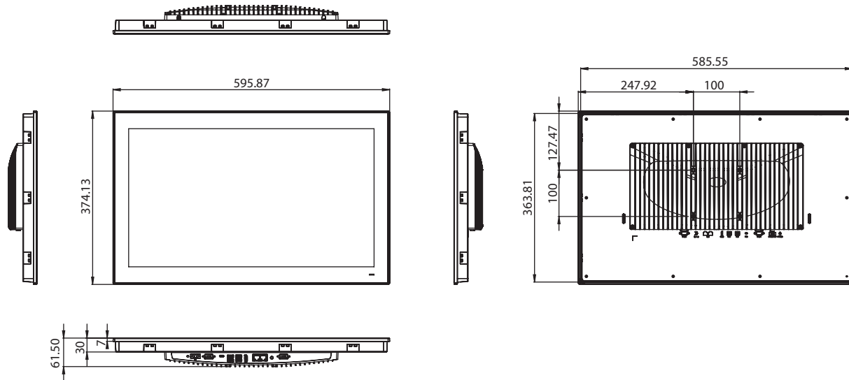
Panel Cutout Dimensions: 586.5 x 364.8 mm (23.09 x 14.36 in)
