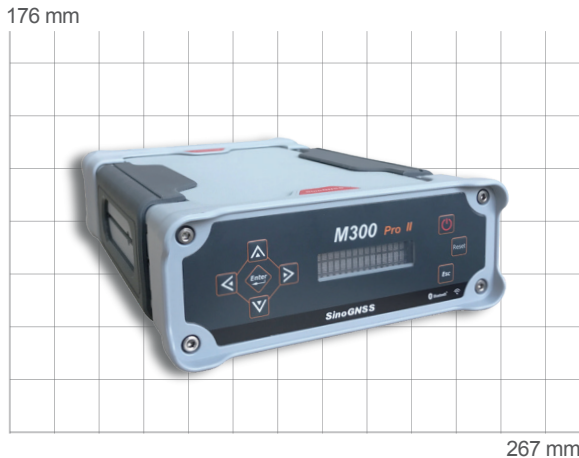
Size: 267 mm × 176 mm × 67 mm Weight: 2.83 kg
